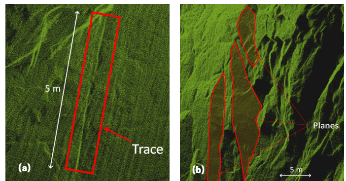
Example point cloud density from Hovermap provides sufficient detail for the recognition of (a) structural discontinuity traces and (b) planes.
