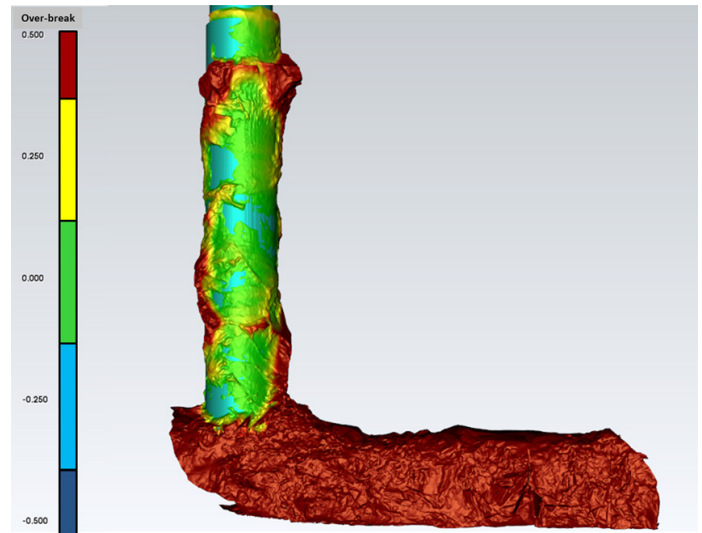
Example of overbreak analysis from a Hovermap shaft scan. The data illustrating both the location and severity of observed issues.
