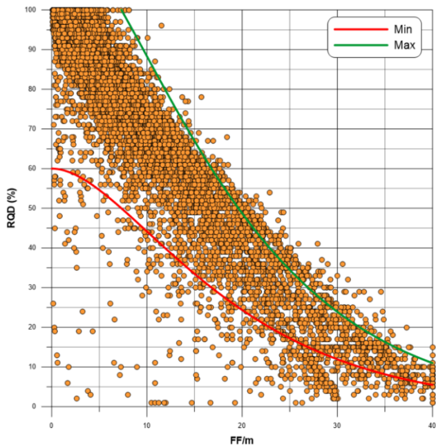
Figure 2. RQD vs. FF/m correlation. Most of the data are in the confidence range defined by Priest & Hudson [16].
