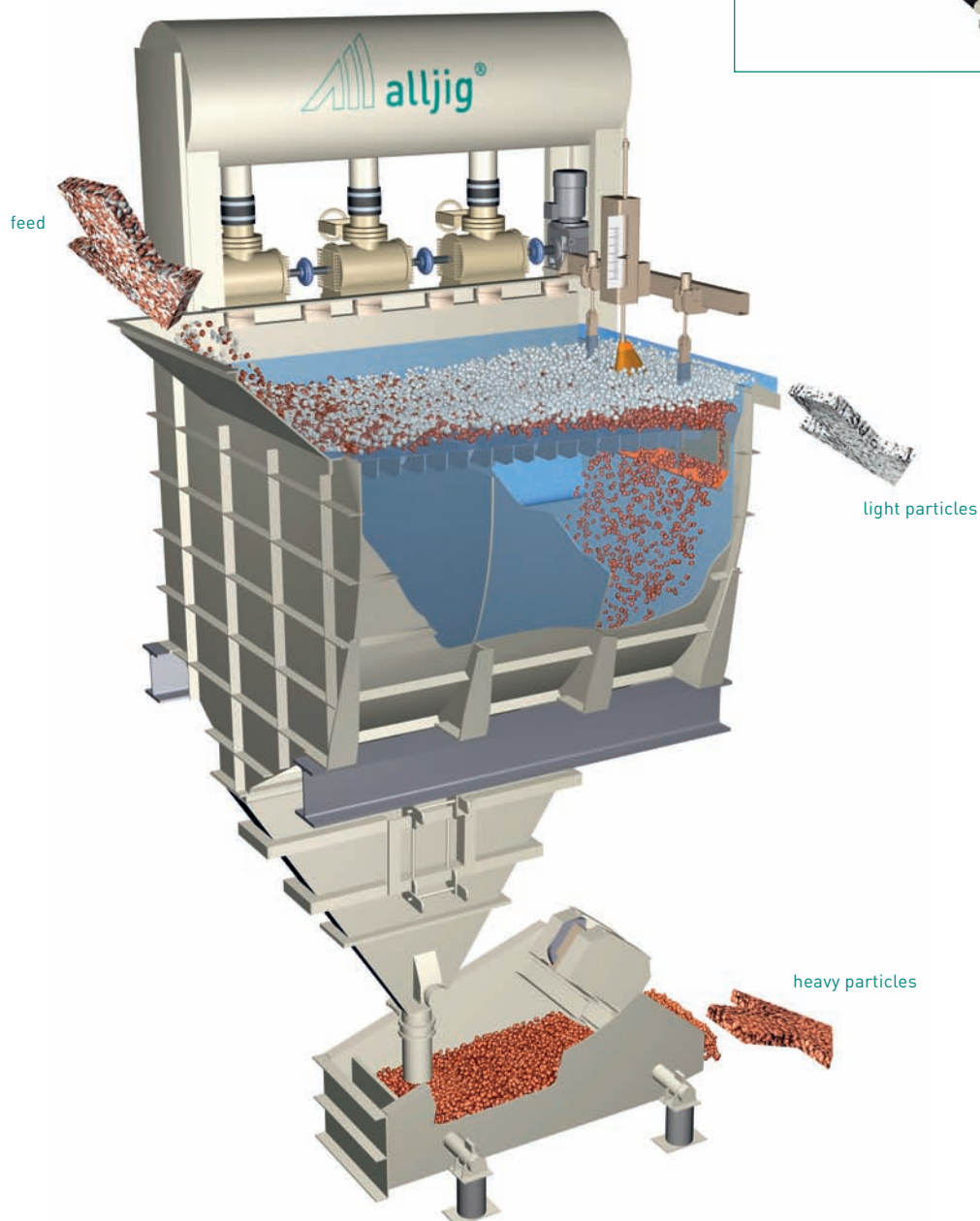
alljig®-GR grain size max. 100mm (4")
