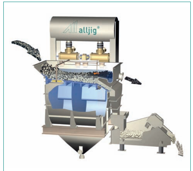
alljig®-GR grain size max. 100mm (4")
