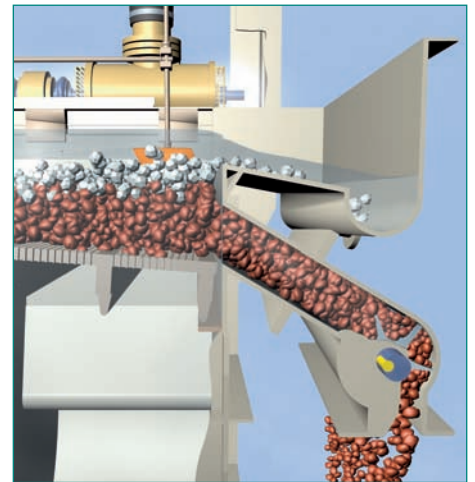
Star gate discharge , grain size max. 60mm (2")
