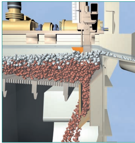
Bottom gate , grain size max. 25mm (1")
